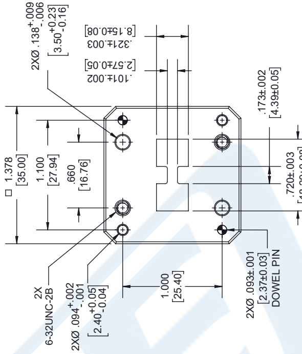
FLANGE DETAIL
