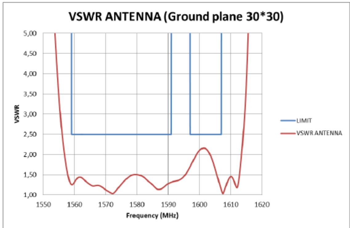
Figure 1: VSWR
