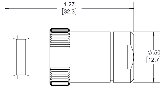
BNC FEMALE
