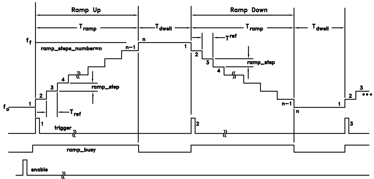
Figure 3. 2-Way Sweep Control via Trigger
