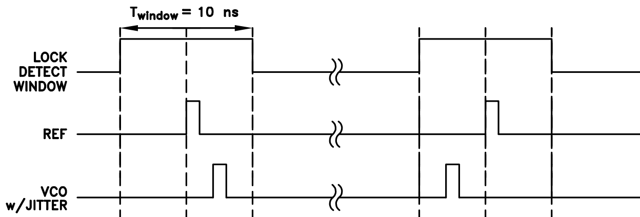
Figure 9. Normal Lock Detect Window
