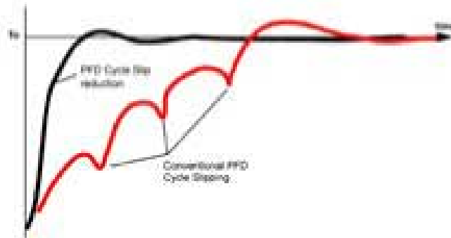
Figure 7. Cycle Slip Prevention (CSP)
