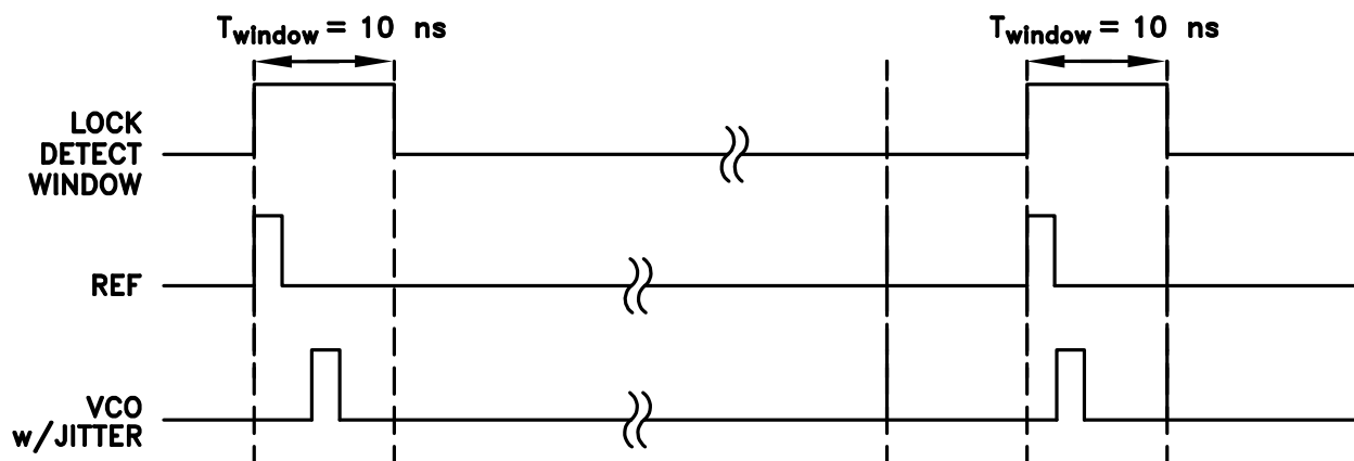
Figure 10. Delayed Lock Detect Window
