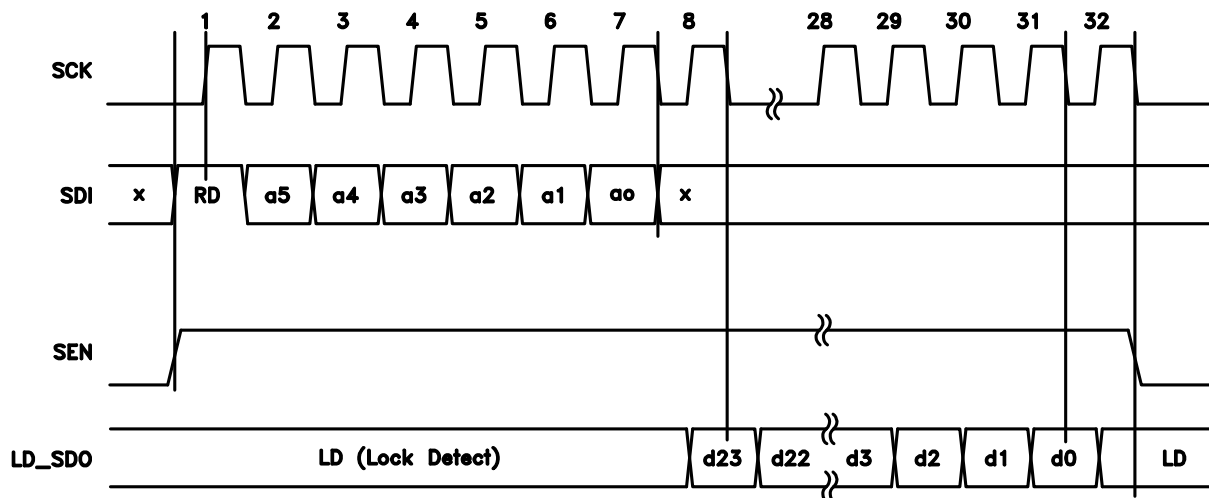
Figure 6. Serial Port Timing Diagram – READ
